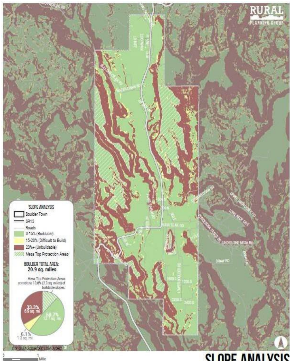
Figure 5. Slope Analysis
